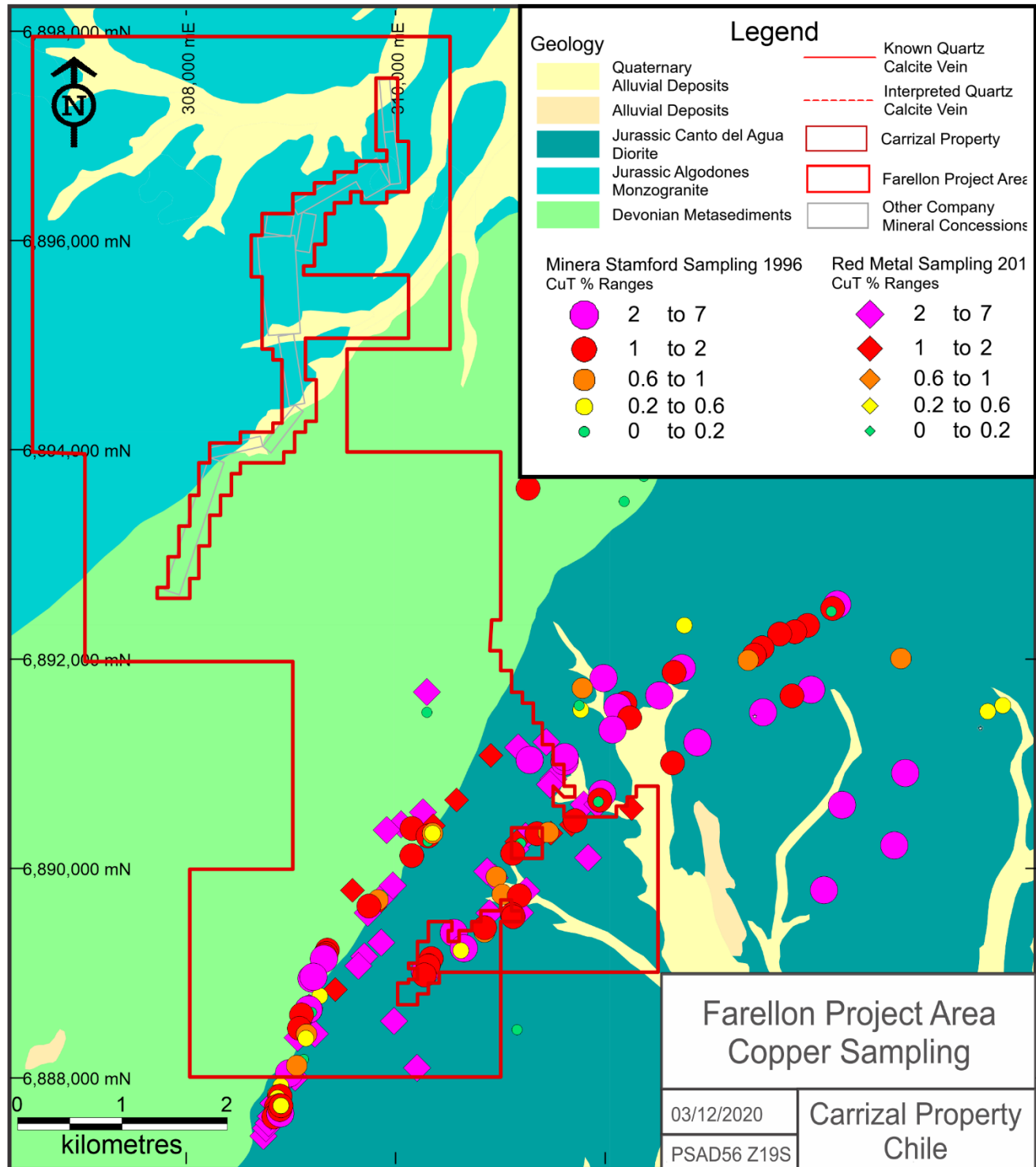
Figure 14 - Results of sampling programs in the Farellón Project area, showing copper concentrations (Geology based on Arevalo and Welkner, 2003; figure provided by Red Metal).
