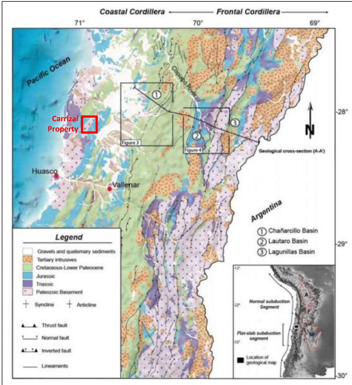
Figure 10 - Generalized geological map of a segment of northern Chile showing the approximate location of the Carrizal Property (outlined in red) (from Martinez et al., 2017).
