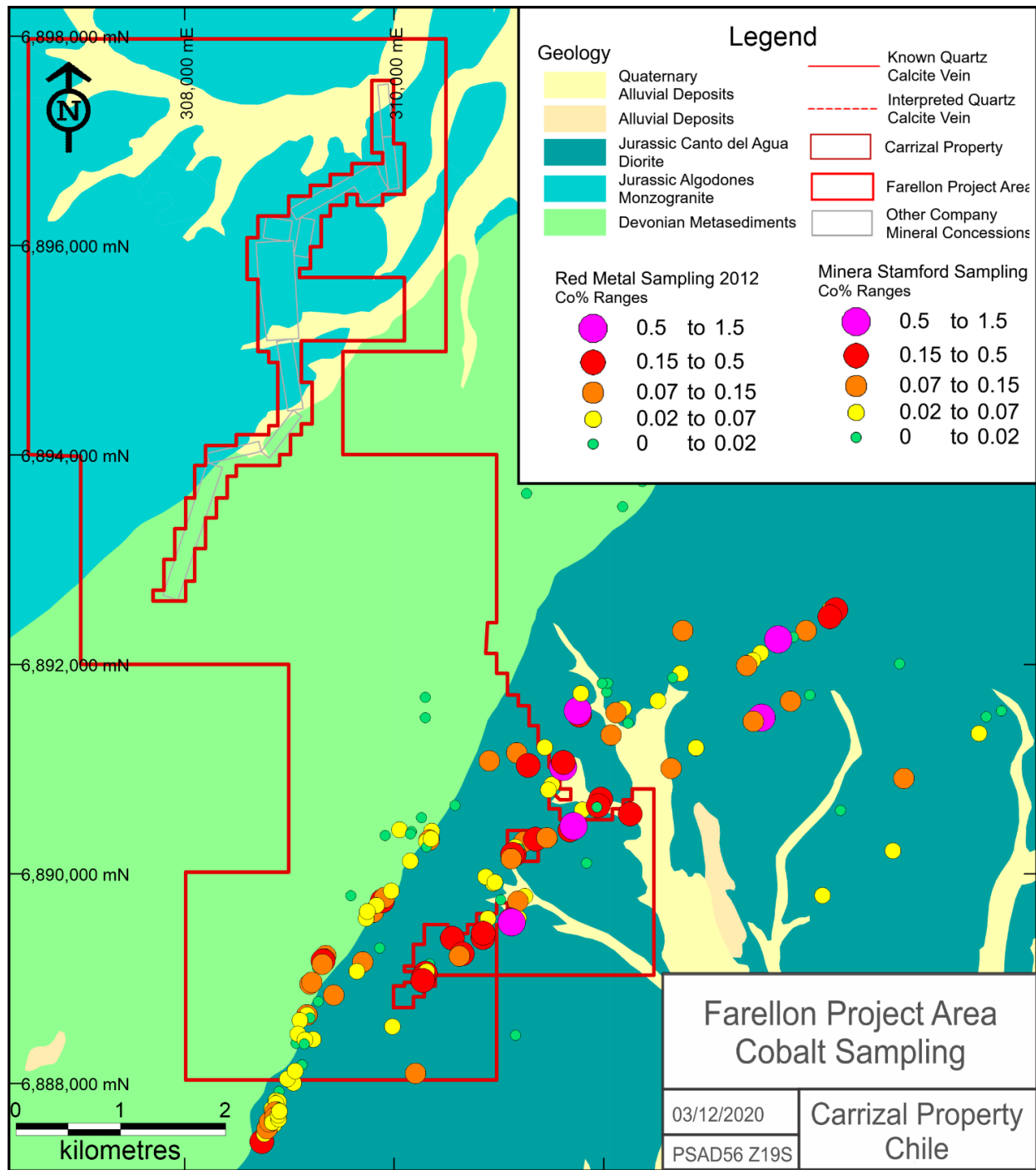
Figure 16 - Results of sampling programs in the Farellón Project area, showing cobalt concentrations (Geology based on Arevalo and Welkner, 2003; figure provided by Red Metal).
