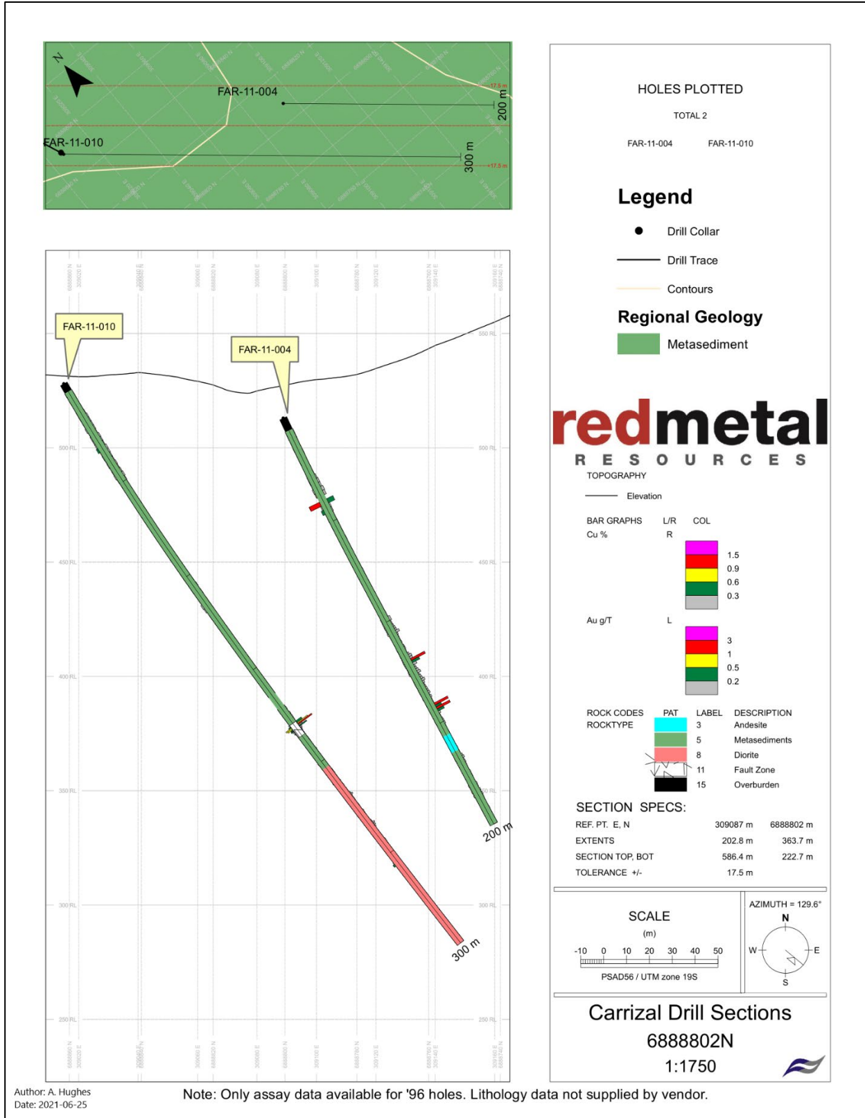
Figure 25 - Drill hole section for FA-11-004 and -010 (figure provided by Red Metal)
