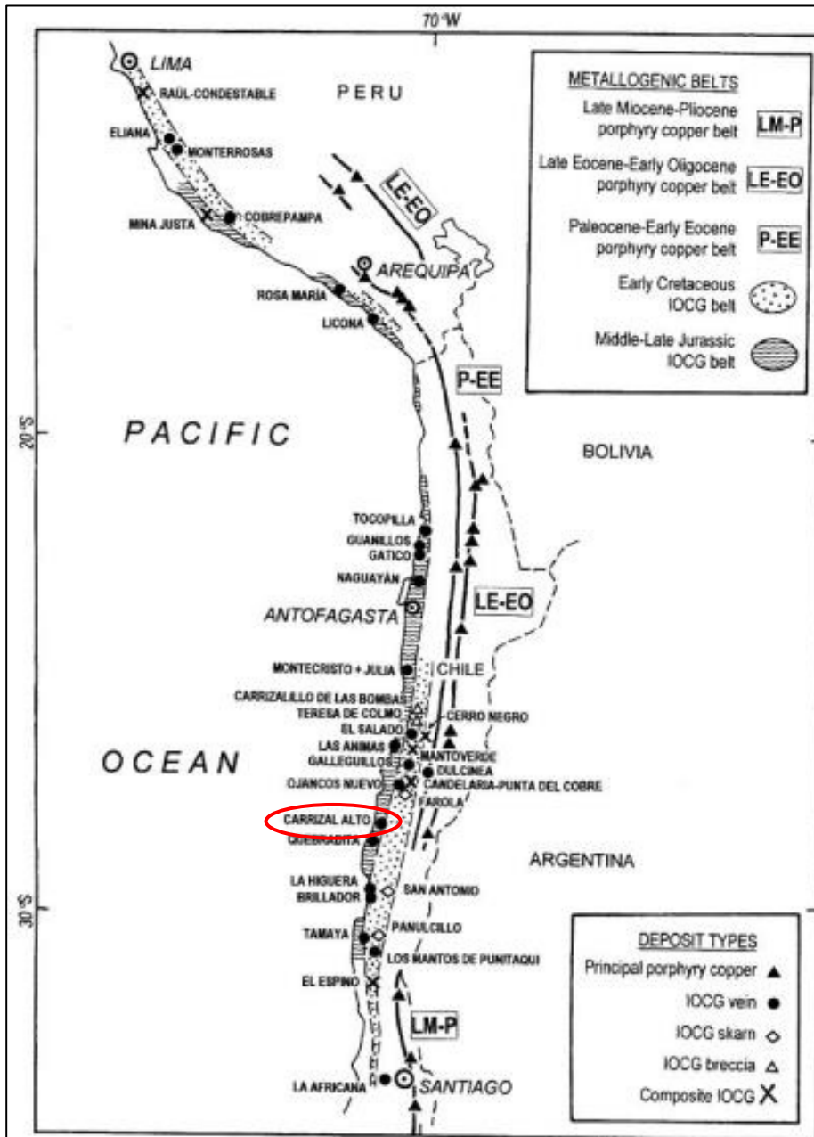
Figure 13 - The Central Andean IOCG Province of northern Chile (Sillitoe, 2003). The Carrizal Alto Mine, directly adjacent to the Carrizal Cu-Co-Au Property, is highlighted (red oval) for reference.
