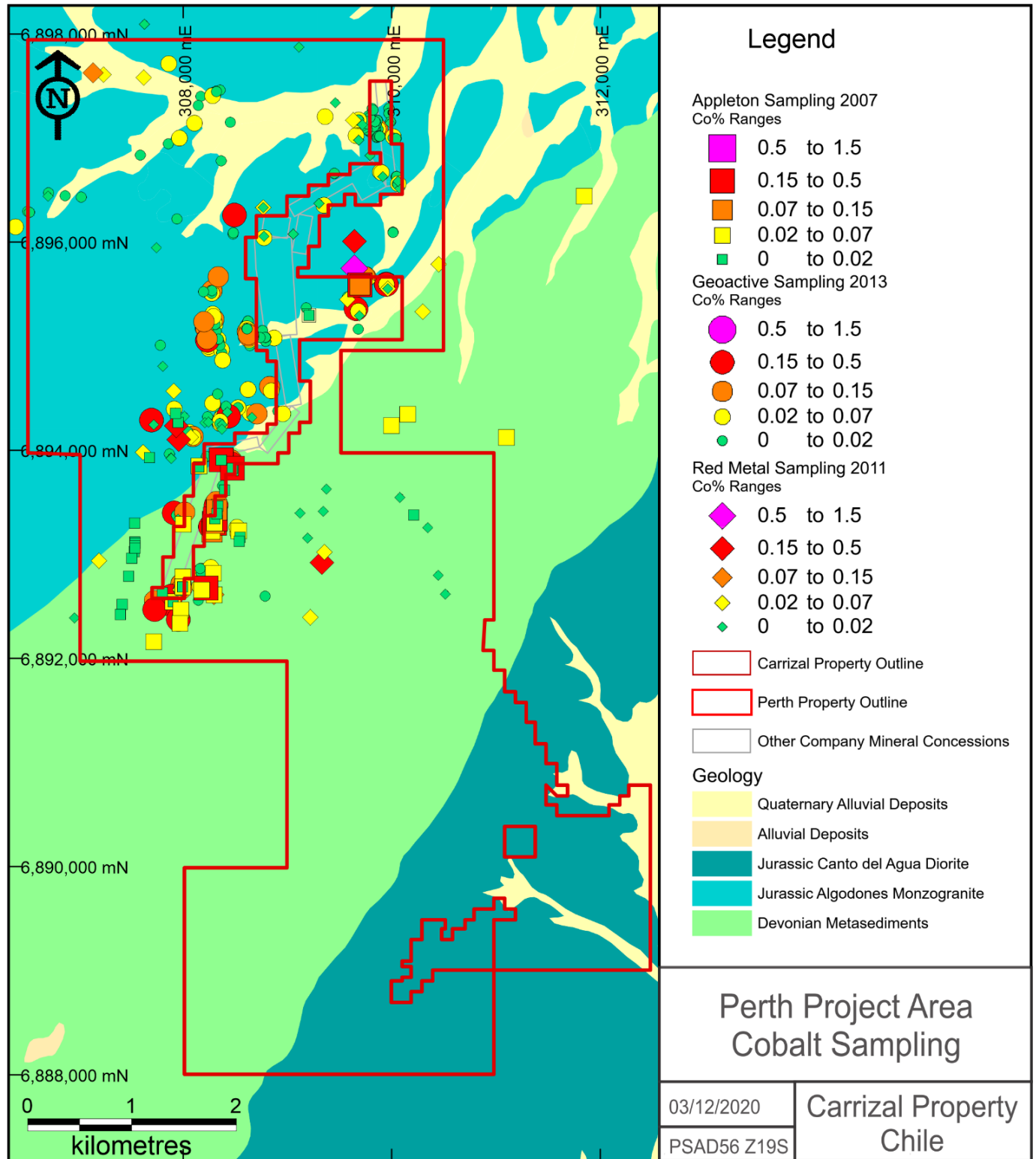
Figure 20 - Results of sampling programs in the Perth Project area, showing cobalt concentrations (Geology based on Arevalo and Welkner, 2003; figure provided by Red Metal).
