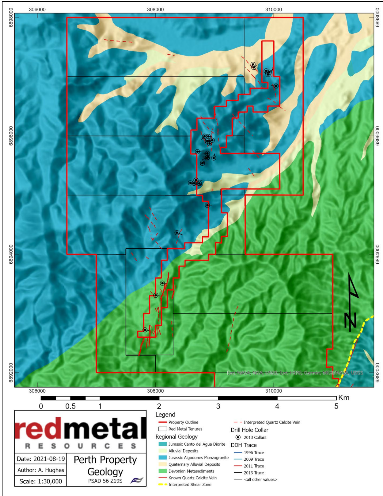
Figure 17 - Perth Geology and Veining (Geology based on Arevalo and Welkner, 2003; figure provided by Red Metal).
