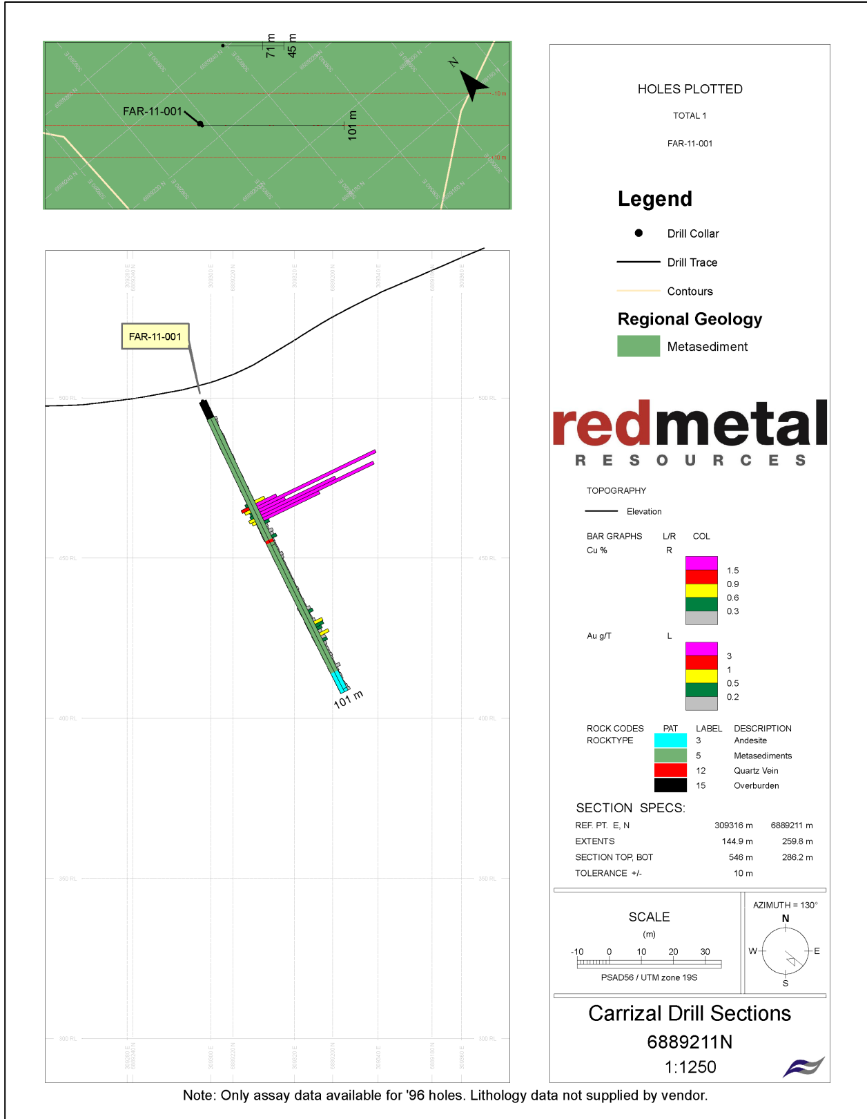
Figure 22 - Drill hole section for FA-11-001 (figure provided by Red Metal).
