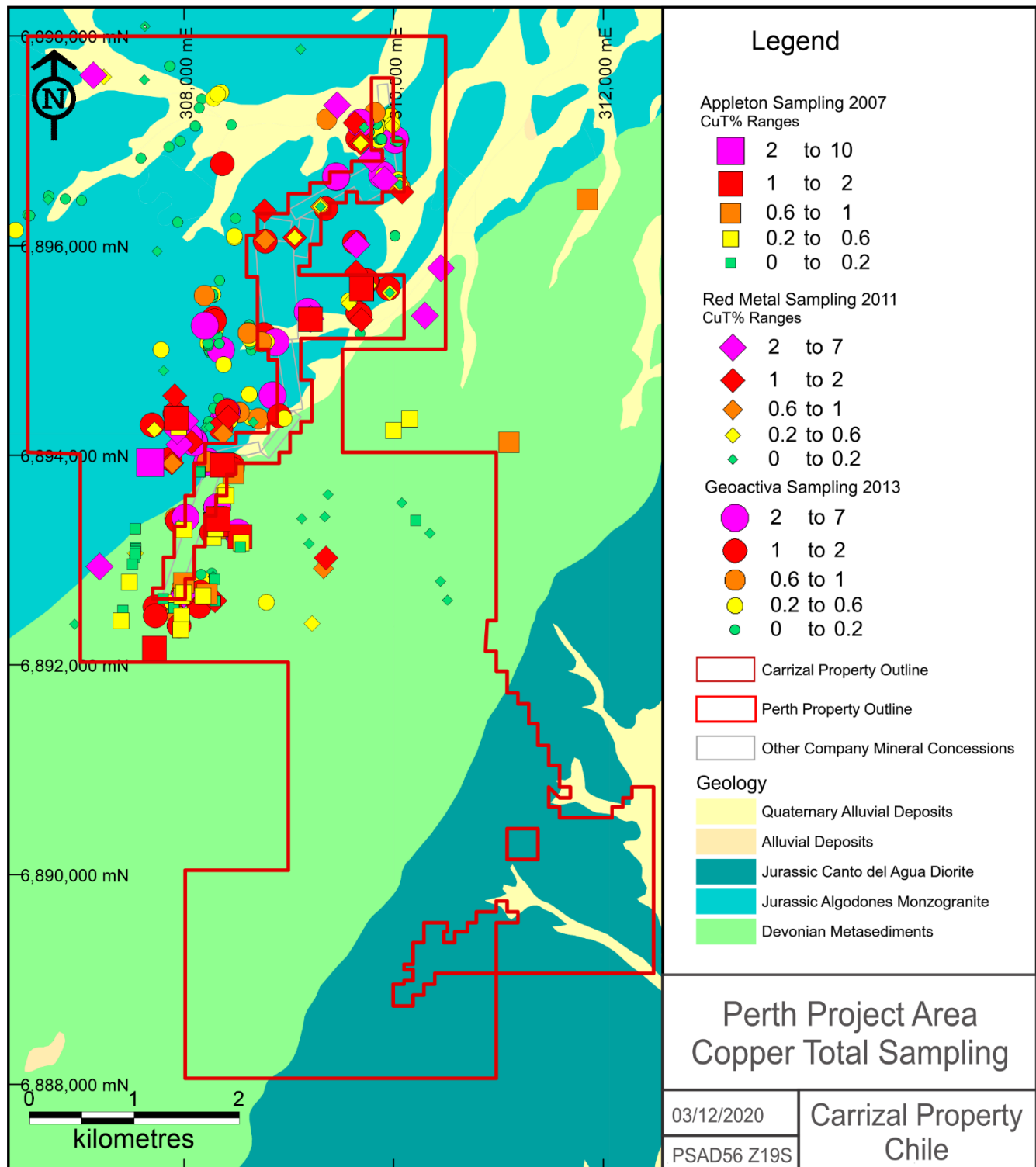
Figure 18 - Results of sampling programs in the Perth Project area, showing copper concentrations (Geology based on Arevalo and Welkner, 2003; figure provided by Red Metal).
