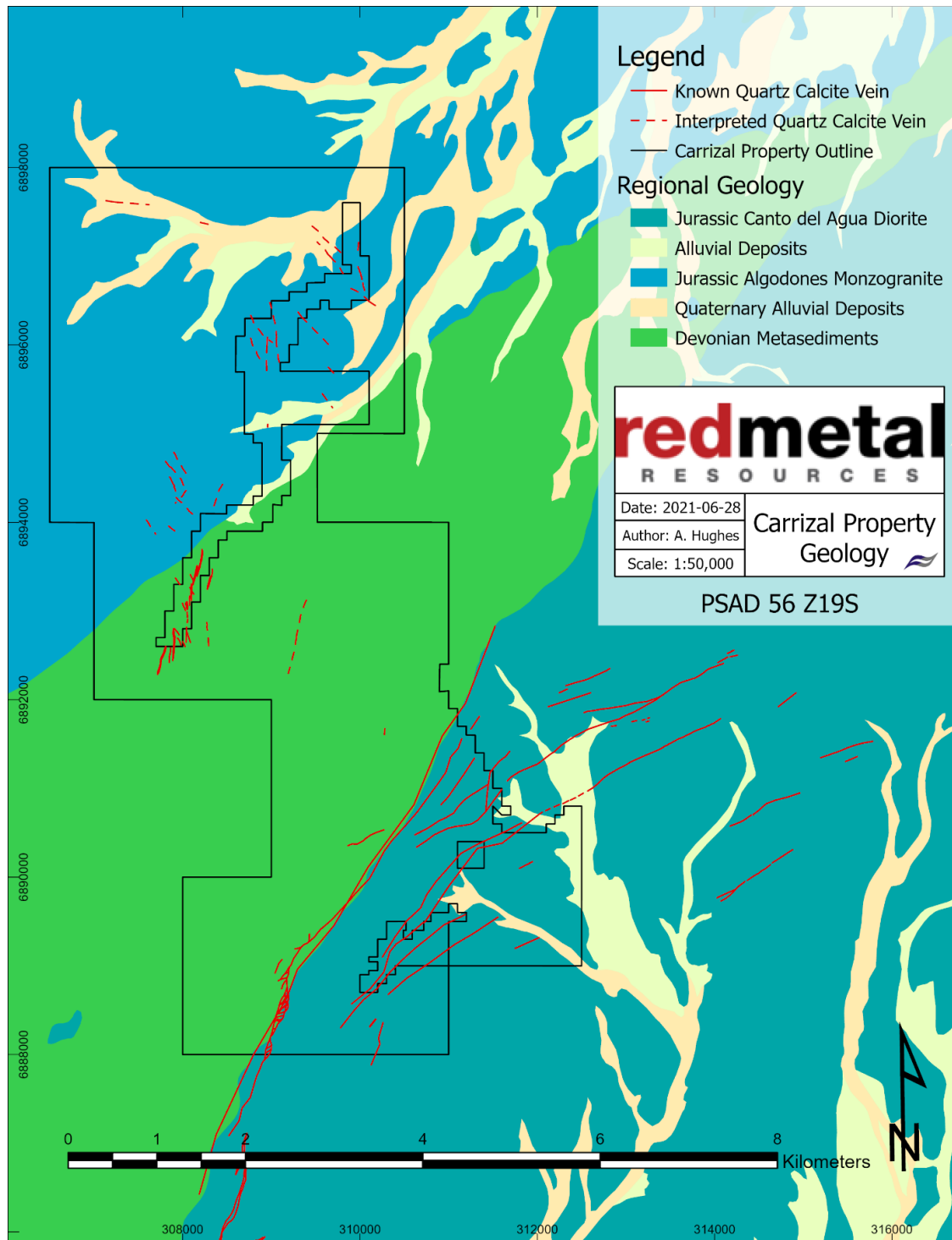
Figure 12 - Property geology of the Carrizal Cu-Co-Au Property, northern Chile (geology after Arevalo and Welkner, 2003; figure provided by Red Metal).
