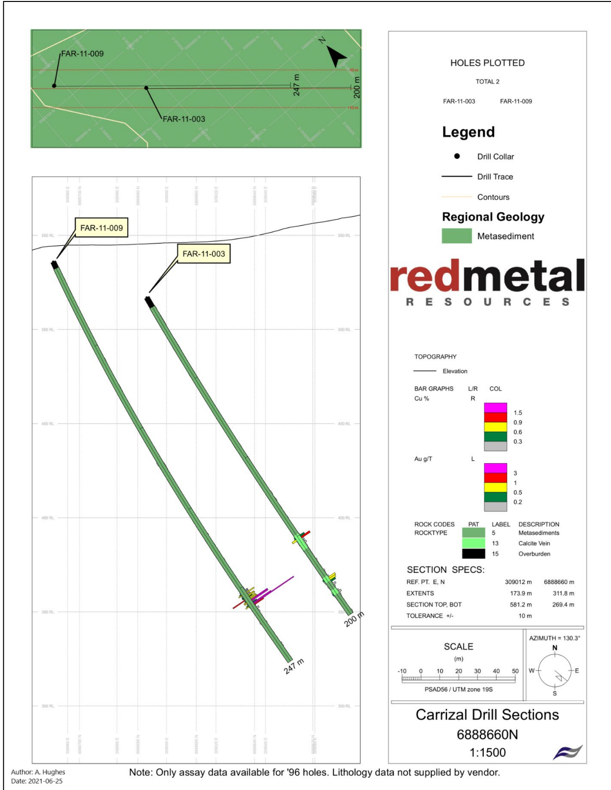
Figure 24 – Drill Section FA-11-003 and -009 (figure provided by Red Metal)
