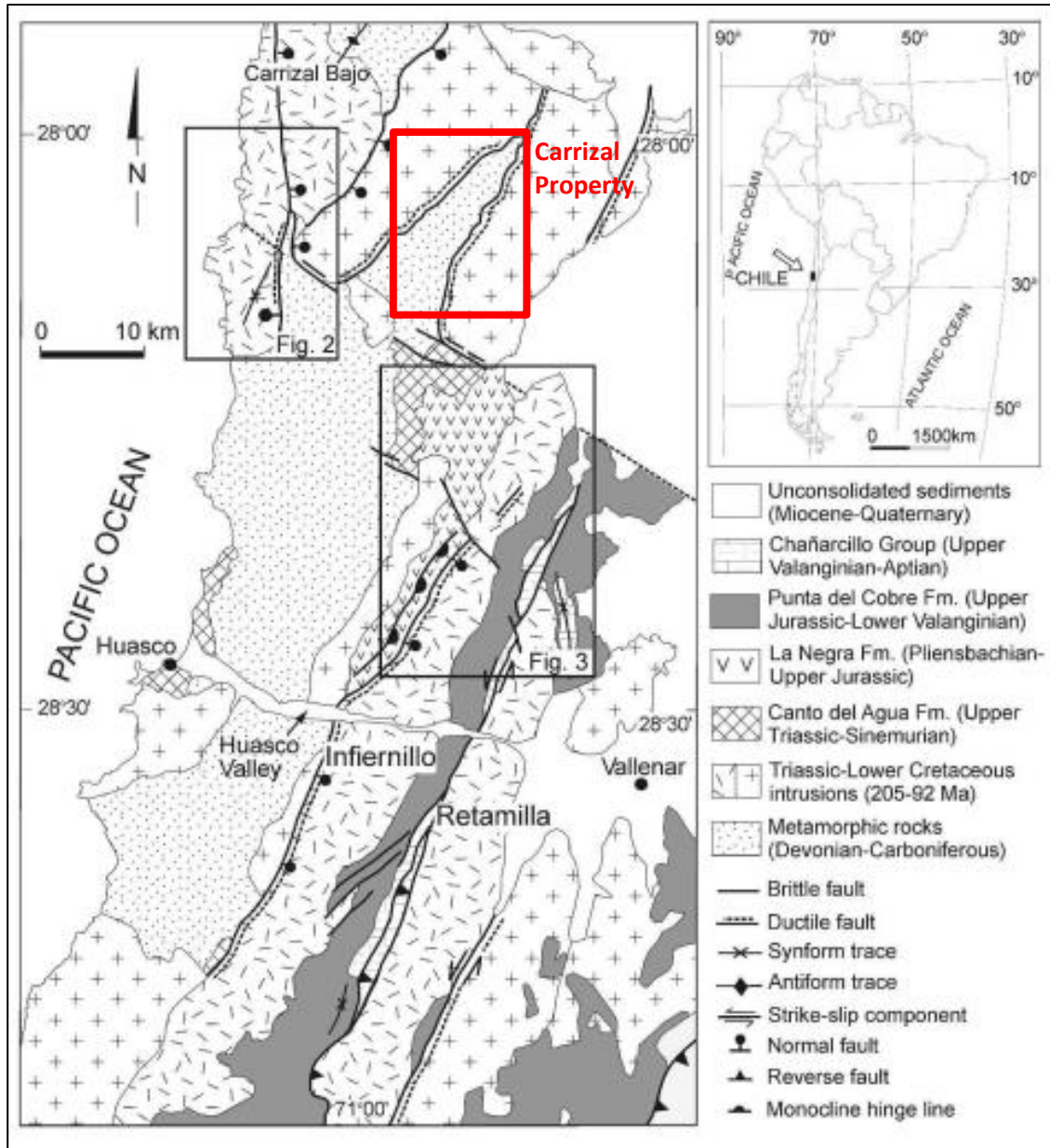
Figure 11 - Local geology surrounding the Carrizal Cu-Co-Au Property (outlined in red) (after Grocott et al., 2009).
