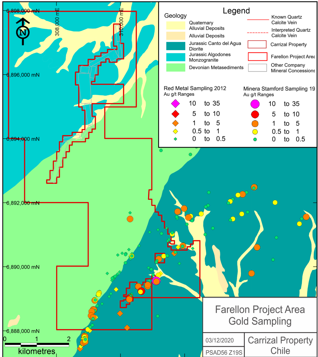
Figure 15 - Results of sampling programs in the Farellón Project area, showing gold concentrations (Geology based on Arevalo and Welkner, 2003; figure provided by Red Metal).
