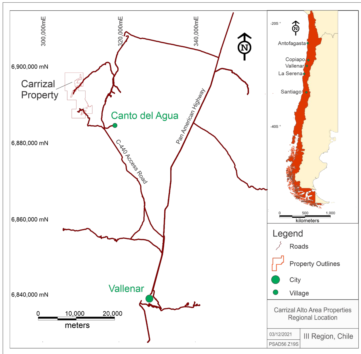
Figure 4 - Location of and access to the Carrizal Cu-Co-Au Property in Region III, Region de Atacama, northern Chile (figure provided by Red Metal).
