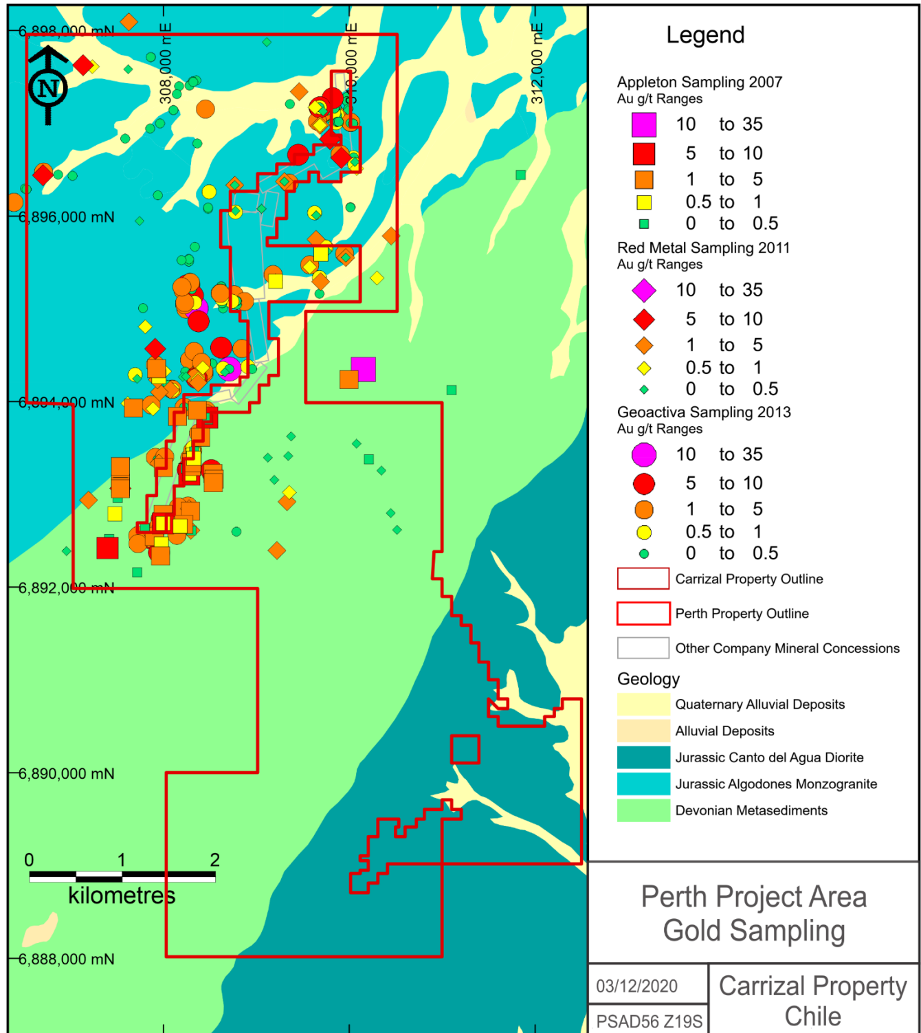
Figure 19 - Results of sampling programs in the Perth Project area, showing gold concentrations (Geology based on Arevalo and Welkner, 2003; figure provided by Red Metal).
