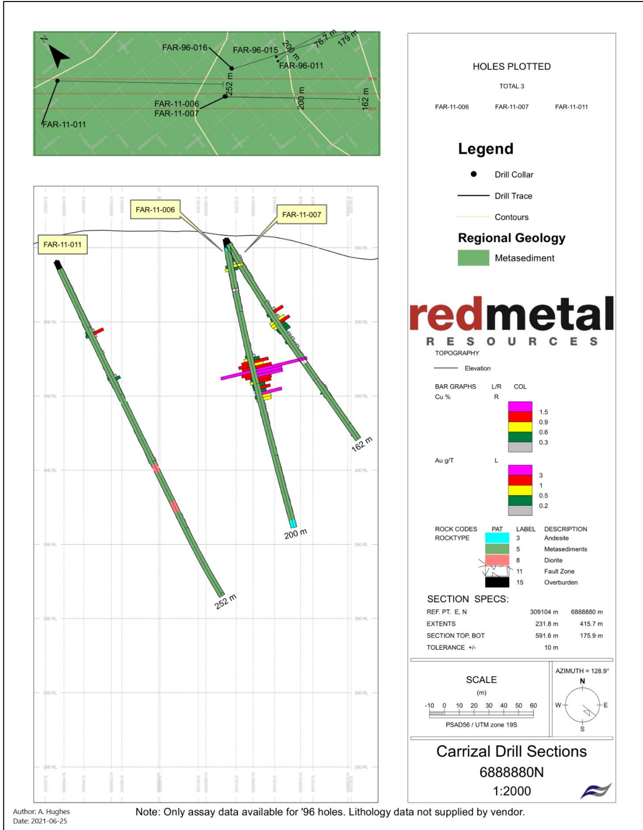
Figure 27 - Drill hole section for FA-11-006, -007, and -011, and historical (figure provided by Red Metal) .
