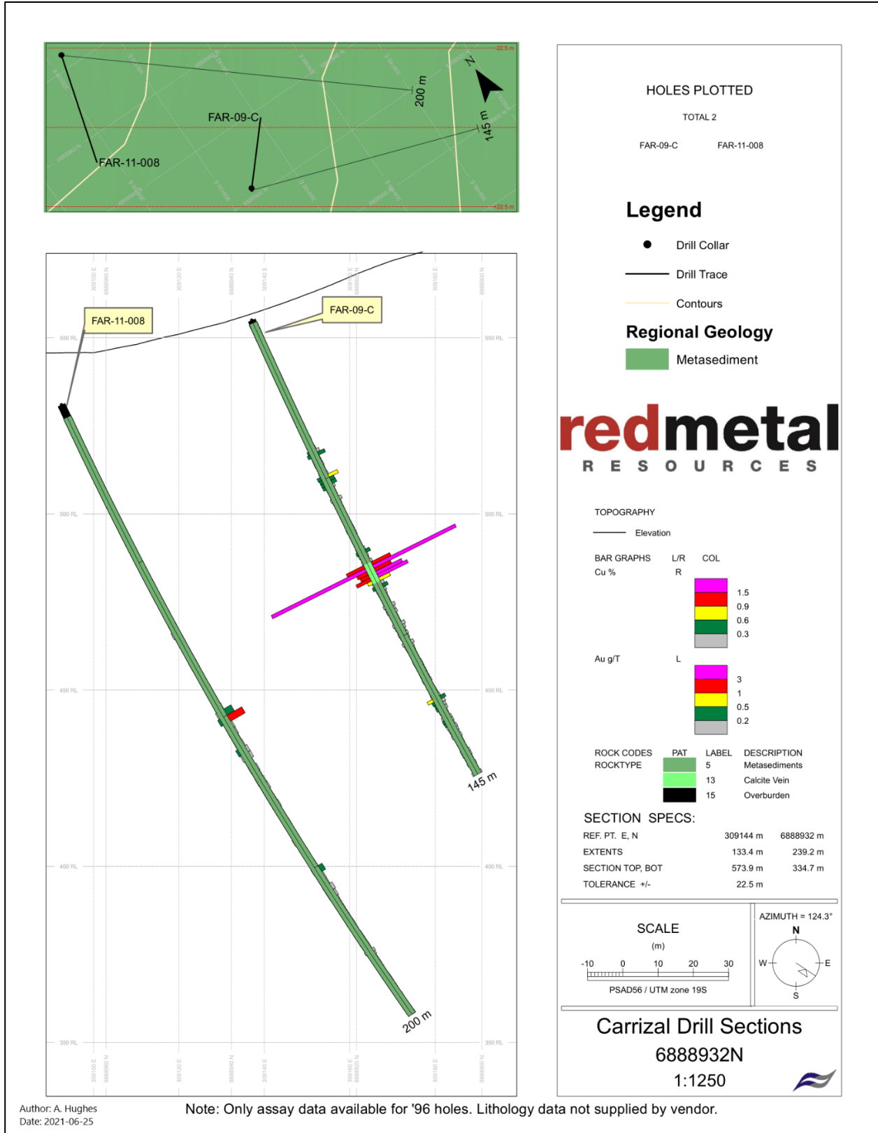
Figure 28 - Drill hole section for FA-11-008, as well as historical holes (figure provided by Red Metal)
