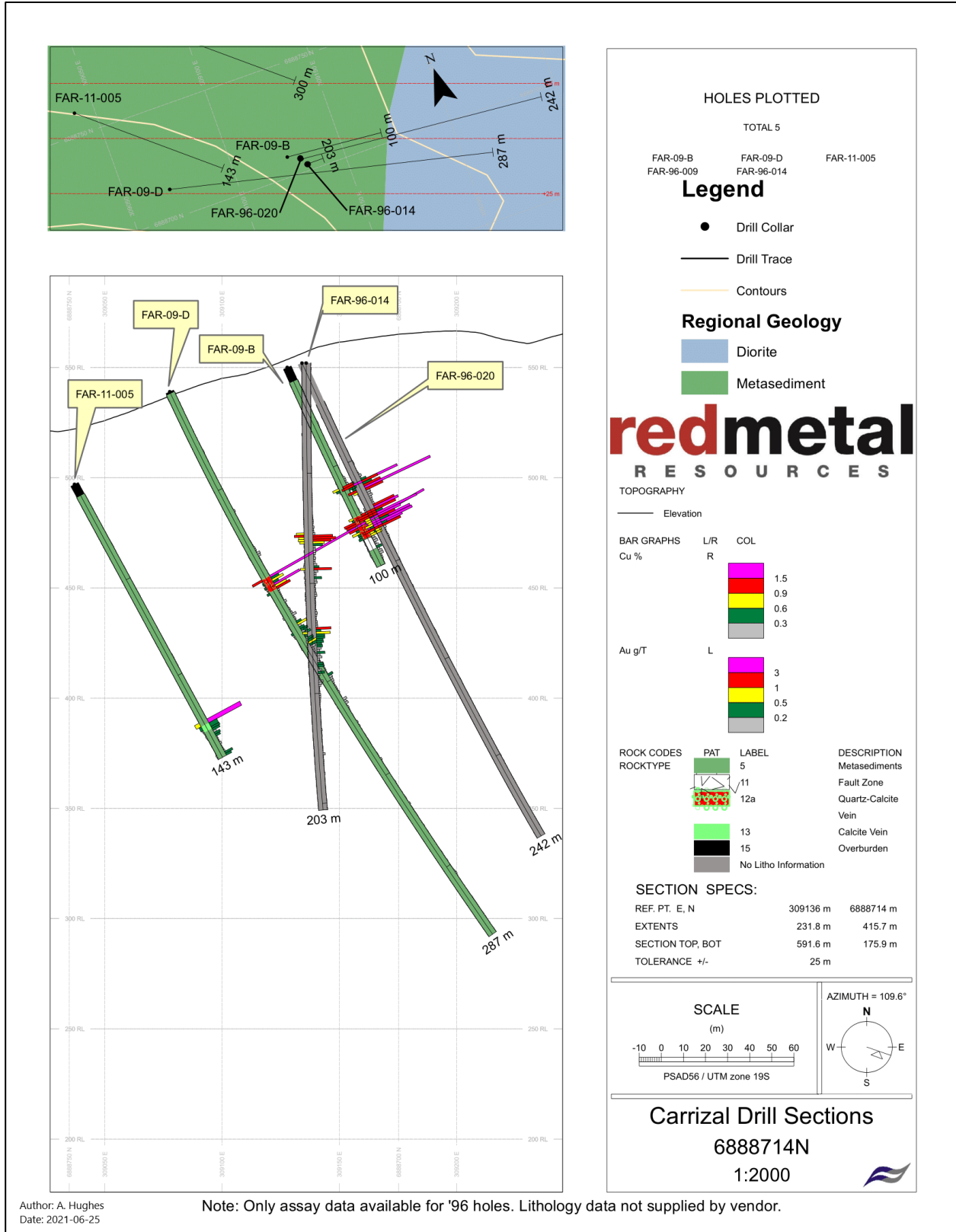
Figure 26 - Drill hole section for FA-11-005 and previous holes (figure provided by Red Metal) .
