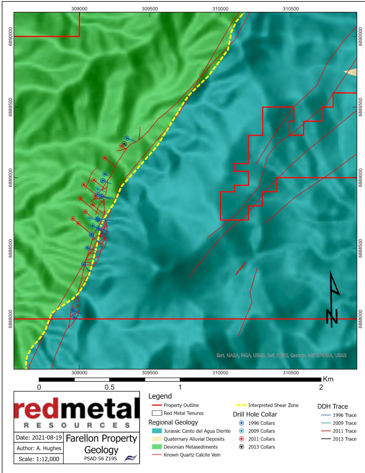
Figure 21 - Farellon Drill Collar Locations (figure provided by Red Metal).
